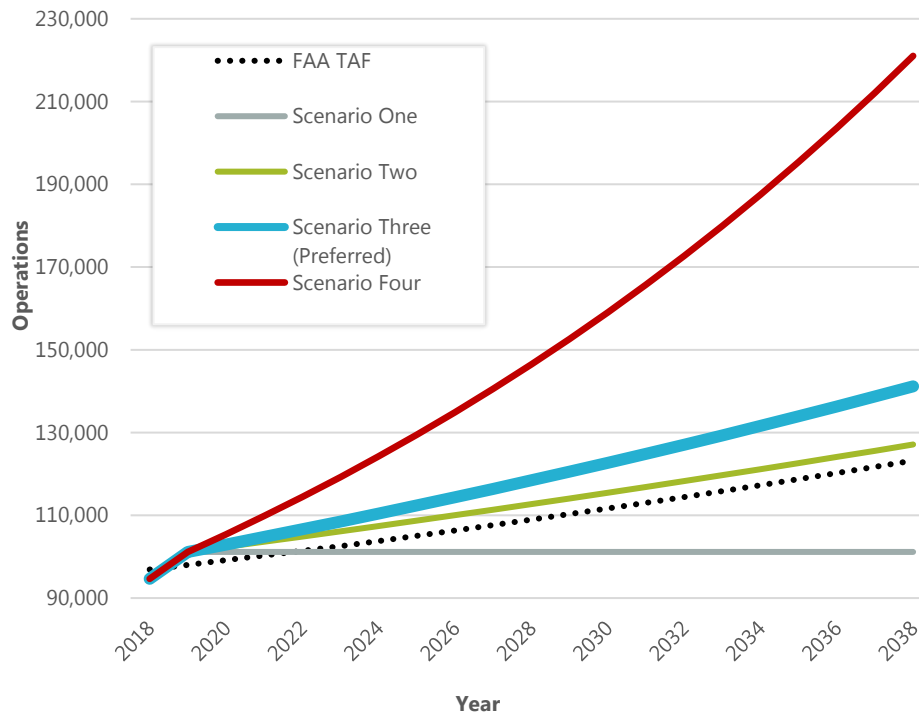
Figure 3-3: GA/Air Taxi Operations Forecasts, 2018-2038
